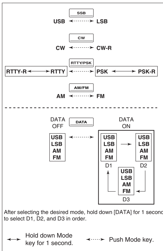
Mode keys
